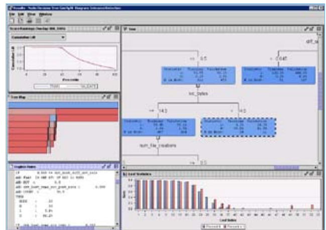
Develop decision trees interactively. Numerous assessment plots to help gauge overall tree stability are included.
