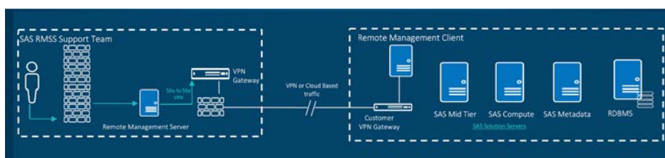
Figure 1: SAS Remote Managed Services architecture with VPN or cloud based traffic.
