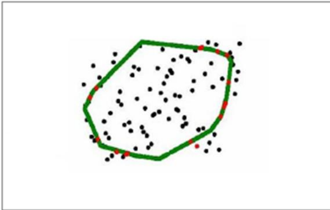
Depth=5 contour. The result of the combination of Genetic and Shake-and-Bake algorithms on a set of 100 data points
