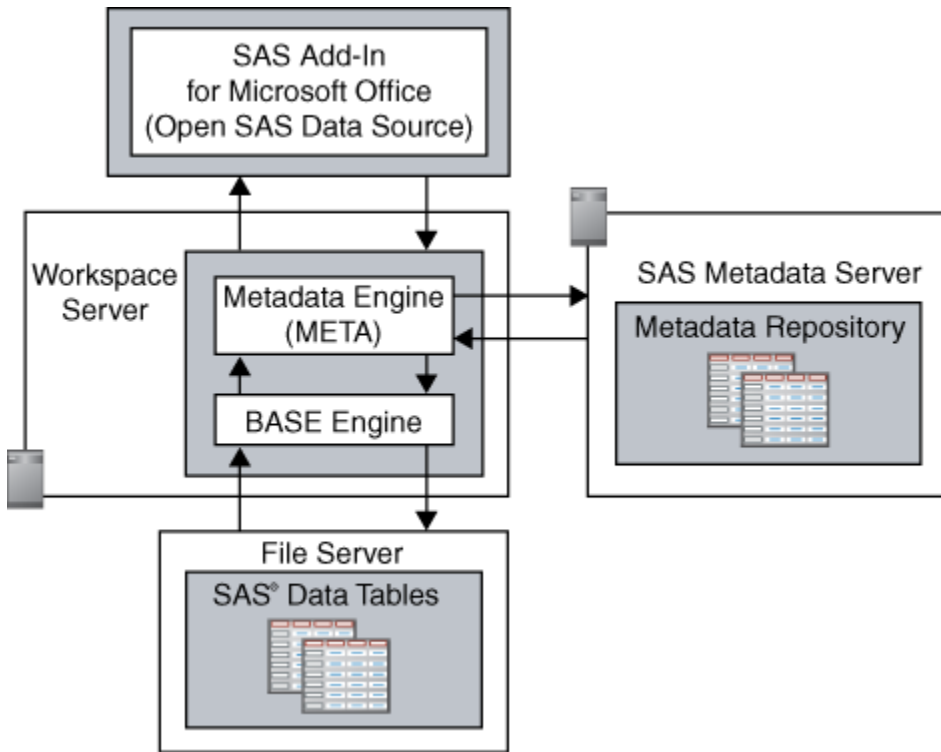
Display 3.1 Metadata Engine Invocation of the Base SAS Engine
